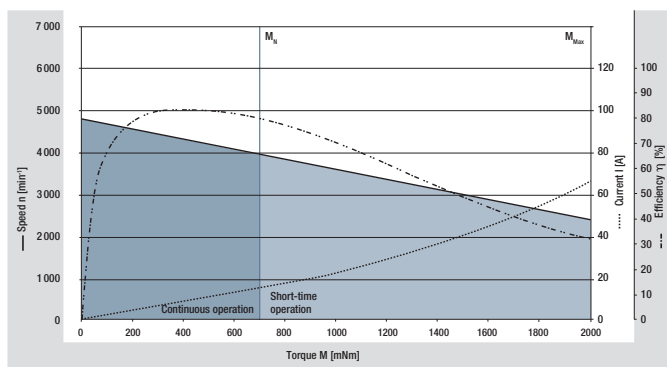
A ECI-80.20-K1, 24 V (at 25 °C)
