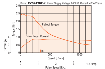
PKP268D42A2/PKP268D42B2
