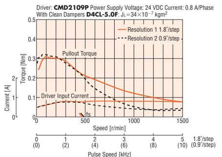
PKP244U08A/PKP244U08B
