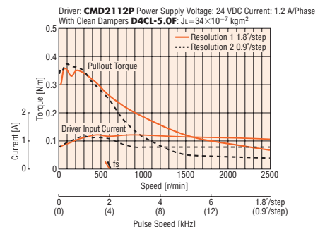
PKP244U12A/PKP244U12B
