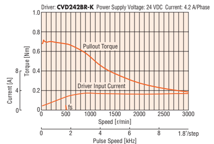
PKP266D42A2-R2EL/ PKP266D42A2-R2FL
