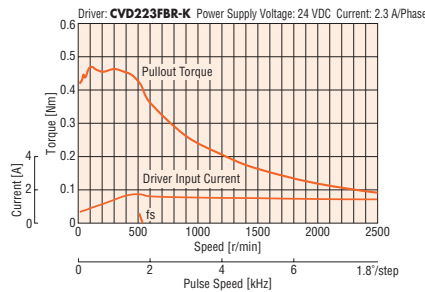
PKP245D23A2-R2EL/PKP245D23A2-R2FL
