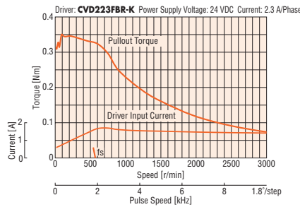
PKP244D23A2-R2EL/PKP244D23A2-R2FL
