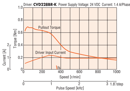
PKP266D14A2-R2EL/ PKP266D14A2-R2FL
