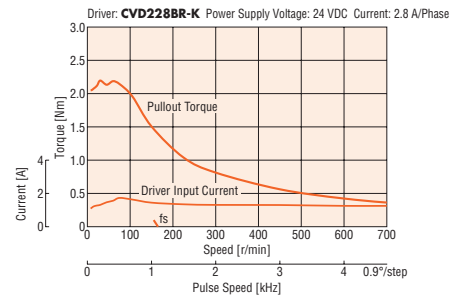
PKP268MD28A2/ PKP268MD28B2
