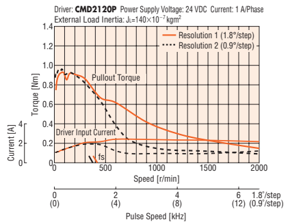
PKP266U20A2-R2EL/PKP266U20A2-R2FL
