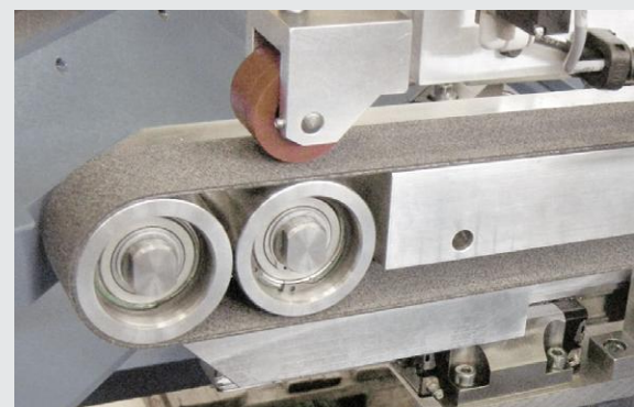
Conveying of punched metal sheets VV06 E
